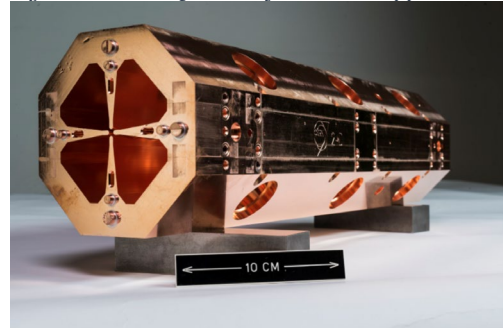
Figure 6 HF-RFQ module for medical applications
